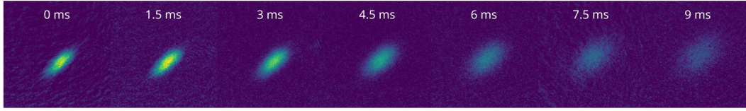
Figure 7.3. TOF images of the atomic cloud after release from the red MOT, taken at increasing expansion times from 0 to 9 ms. The growth of the cloud size with TOF is used to extract the temperature via Gaussian fits to the optical density profiles.
