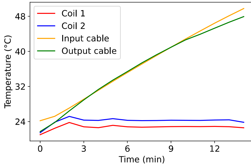
Figure 6.10. Thermal response of coil and cable components under a constant 190 A current. The plot shows temperature variations recorded by four sensors over time.
