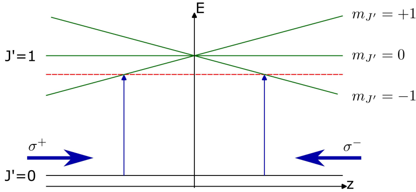
Figure 2.2. Zeeman splitting of the excited state J' = 1 in the presence of a magnetic field gradient. Two counter-propagating circularly polarized beams drive \sigma^+ and \sigma^- transitions from the ground state J = 0 . The differential Zeeman shifts make one beam closer to resonance depending on the atomic position, generating a restoring force toward the magnetic-field zero.
