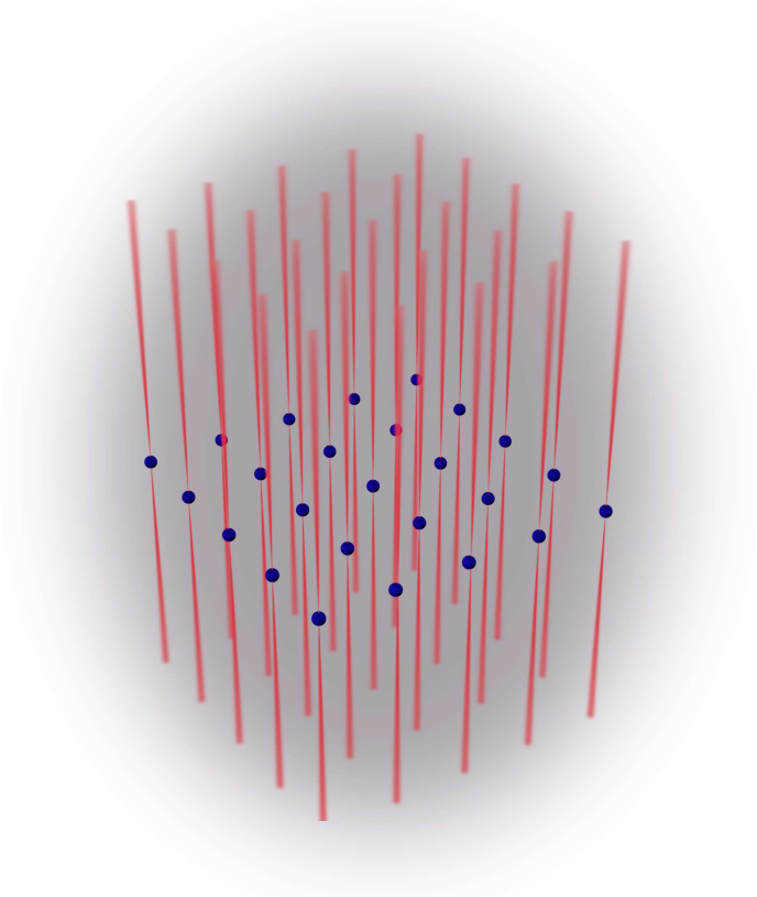
Figure 1.2. Schematic representation of an Array of optical tweezers (red beams) trapping individual atoms (blue spheres).
