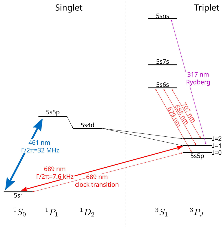
Figure 3.1. Simplified energy scheme for ^{88}\text{Sr} , with transitions of interest shown.
