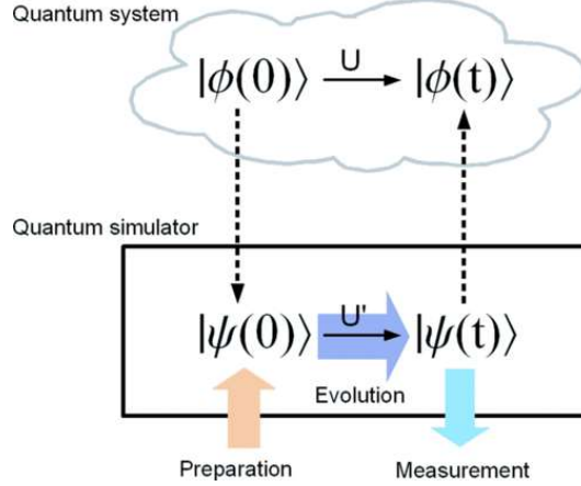
Figure 1.1. Schematic representation of a quantum system and its corresponding quantum simulator. The quantum state |\varphi(0)\rangle evolves into |\varphi(t)\rangle via the unitary transformation U = \exp\{-i\hbar H_{\text{sys}}t\} . The quantum simulator evolves from the state |\psi(0)\rangle into |\psi(t)\rangle via U' = \exp\{-i\hbar H_{\text{sim}}t\} . The simulator is designed to reproduce the behavior of the simulated system through specific mappings: |\varphi(0)\rangle \leftrightarrow |\psi(0)\rangle , |\varphi(t)\rangle \leftrightarrow |\psi(t)\rangle , and U \leftrightarrow U' . While the simulated system may be uncontrollable or experimentally inaccessible, the simulator is fully controllable: the initial state |\psi(0)\rangle can be prepared, the unitary evolution U' can be engineered, and the final state |\psi(t)\rangle can be measured. The result of this measurement provides information about the simulated system. The colored arrows denote the controllable operations. The solid black arrows describe the time evolution of the system and the simulator. The dashed arrows indicate the correspondence between the quantum states of the simulator and the simulated system. Figure taken from Ref. [1].
