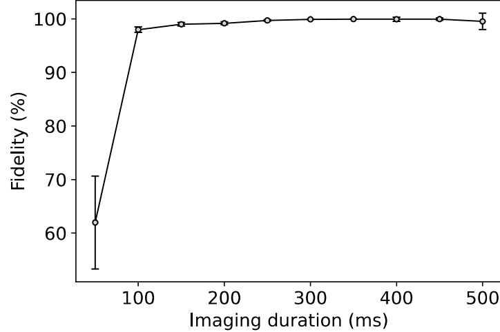
Figure 8.12. Measured imaging fidelity as a function of imaging duration for a fixed trap depth of 360\ \mu\text{K} . Longer exposure times lead to improved photon statistics and higher fidelity, saturating near unity for imaging durations above 250 ms.
