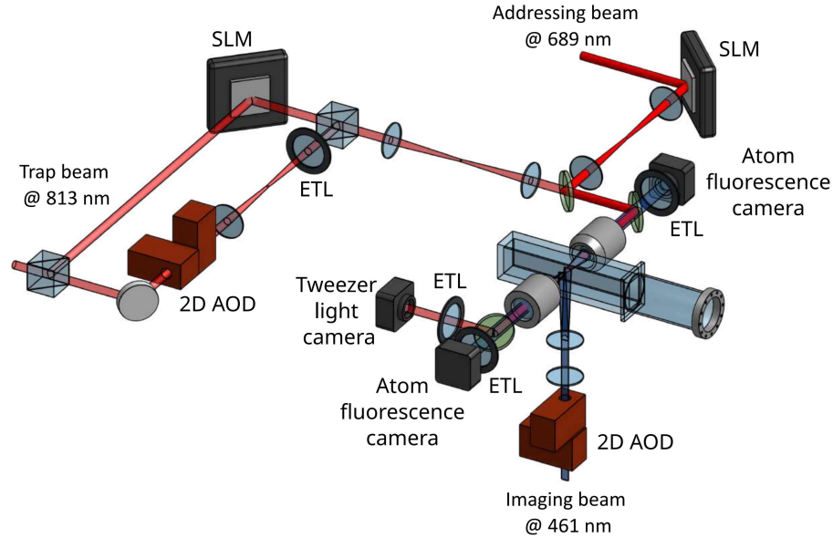
Figure 4.4. Proposed optical layout for the generation and imaging of three-dimensional arrays of optical tweezers. The trapping beam at 813 nm is shaped by a spatial light modulator (SLM) and focused into the vacuum cell through a high-NA objective, which is also used to collect atomic fluorescence. An electrically tunable lens (ETL) in the trapping path allows for axial positioning of the tweezers, while a second ETL in the detection path enables imaging of different planes of the array. A second high-NA objective, aligned from the opposite side, is dedicated to fluorescence collection and imaging of the tweezers, thereby increasing the detection efficiency. Local addressing is provided by a 689 nm beam shaped by an additional SLM. Imaging beams at 461 nm are coupled through acousto-optic deflectors (AODs) to illuminate the atoms for fluorescence detection.
