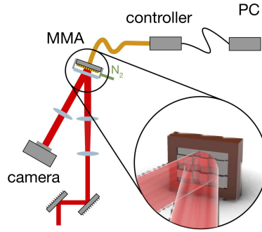
Figure 4.5. The optical setup to generate configurable beam shapes with a phase-only spatial light modulator based on a micro-mirror array (MMA). The generated patterns are characterized on a camera.
