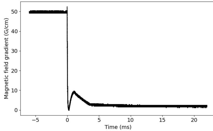
Figure 7.7. Measured magnetic field gradient during the transition from the blue MOT to the red MOT. The gradient is rapidly reduced from 50 \text{ G cm}^{-1} to 2 \text{ G cm}^{-1} by switching off the MOT coils and reactivating them at a lower current. The transient overshoot and subsequent damped oscillations are visible in the measurement of the coil current, taken using a current probe (Danisense DS400UB-10V). Despite the overshoot, the atom capture efficiency in the red MOT remains sufficient for our purposes.
