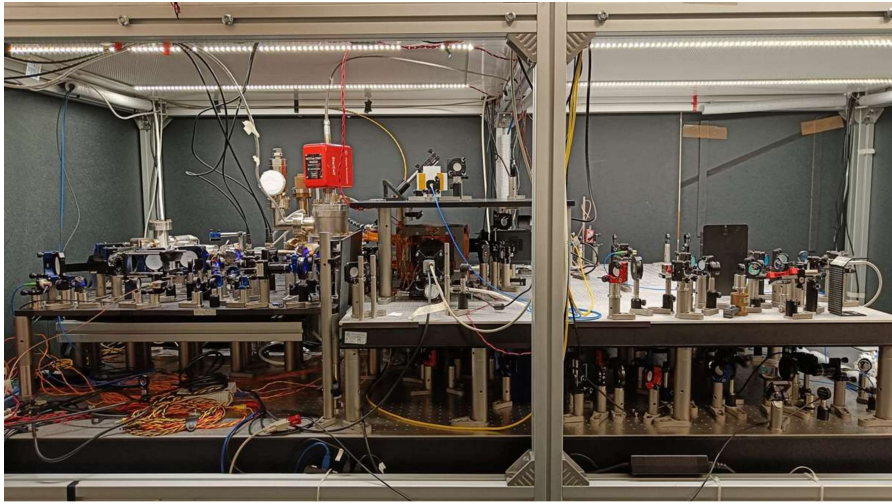
Figure 6.1. Side view of the experimental optical table. On the left side we have the vacuum system, mounted on a separate breadboard on a translation stage. The optical setups for trapping, manipulating and detecting the atoms are assembled on this optical table on three levels.
