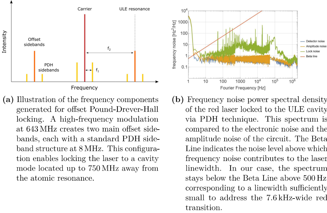
Figure 6.17. 689 nm laser frequency stabilization scheme using PDH locking to a ULE cavity (left) and corresponding frequency noise spectrum (right).
