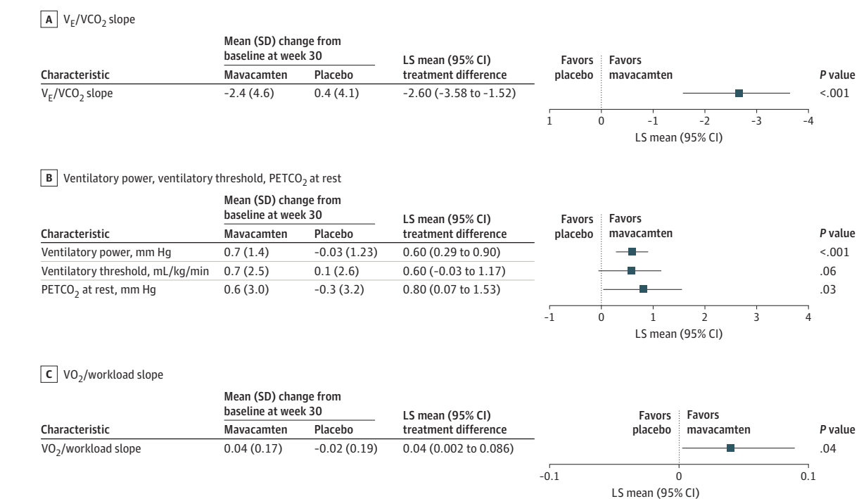
Figure 3. Treatment Difference of the Change From Baseline to Week 30 Between Mavacamten and Placebo in Submaximal Exercise Cardiopulmonary Exercise Testing (CPET) Parameters
