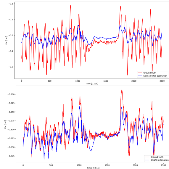
Fig. 1. KF (upside) and DANAE (downside) roll angle estimation compared to the ground truth. This experiment is made on a subsection of the slow walking set of OxIOD.
