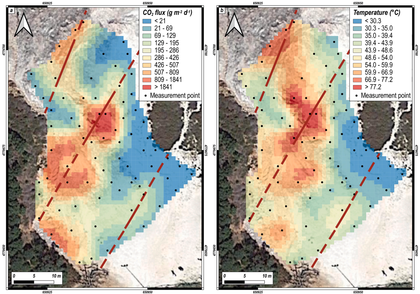
Fig. 7. a) Soil \text{CO}_2 flux, and b) temperature distribution maps. Faults are reported as red lines.
