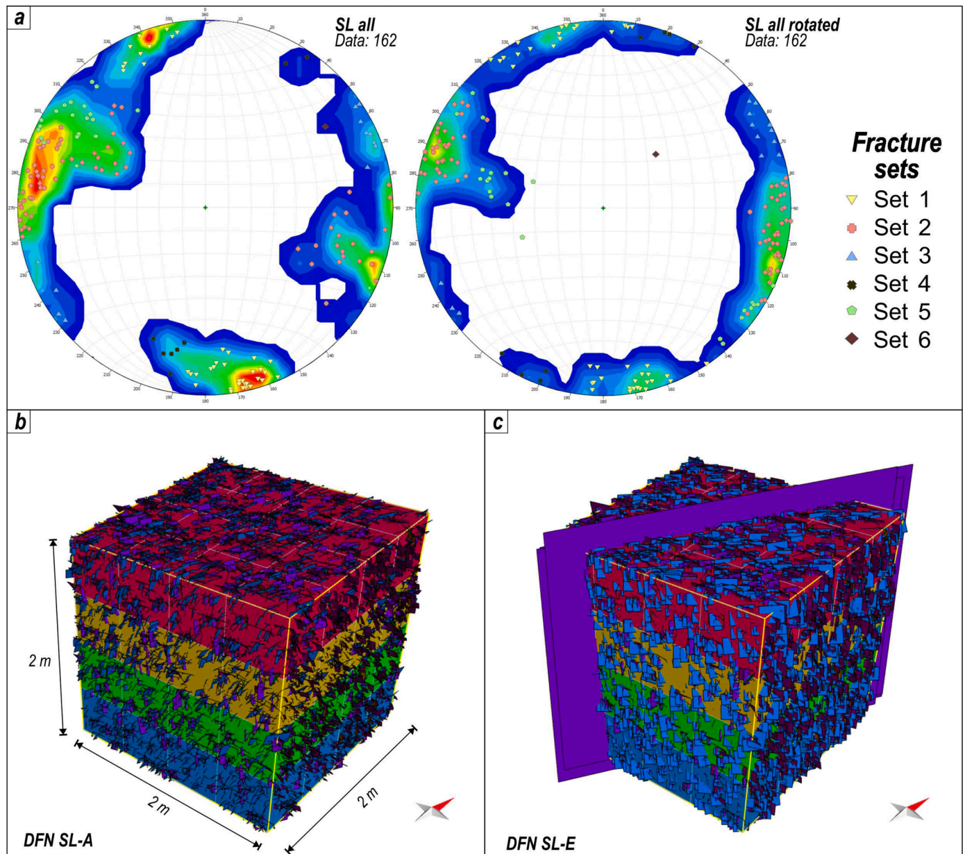
Fig. 11. a) Stereonet data from all the scanlines with and without rotation; b) detail of the DFN models in proximity of the (b) scanlines SL A and (c) SL E. Most of the modelled fractures are stratabound, however near secondary faults non-stratabound fractures parallel to faults N30° striking are present (purple).
