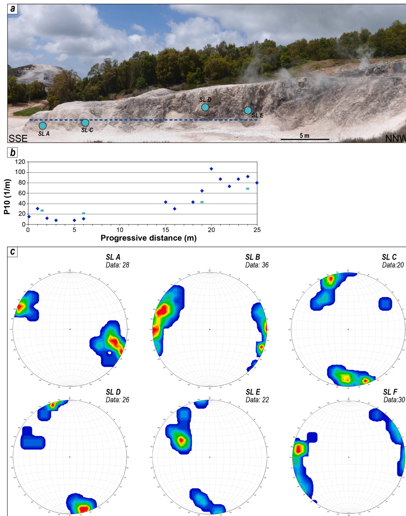
Fig. 9. a) Panoramic view of the scarp where the main scanline (dashed blue line) and the secondary scanlines (SL A, SL C, SL D, SL E) were performed; b) linear fracture intensity P10 along the main scanline indicated in (a); c) stereoplots of the fractures (poles of planes) measured in each of the indicated Scanline.
