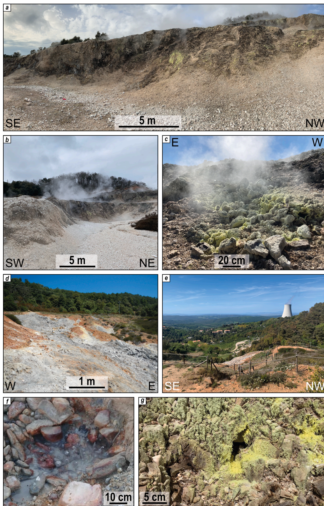
Fig. 4. Field photographs from the Le Biancane natural park. a-b) wall of an abandoned quarry with visible fumaroles and steaming grounds; the rock scarp crosscuts the Monterotondo Marittimo-Sasso Pisano fault zone; c) fumarolic manifestations; d) hydrothermally altered grounds; e) panoramic view of the park with a geothermal power plant cooling tower in the background; f) bubbling pool; g) acicular aggregates and encrustations of native sulfur in a fumarolic vent.
