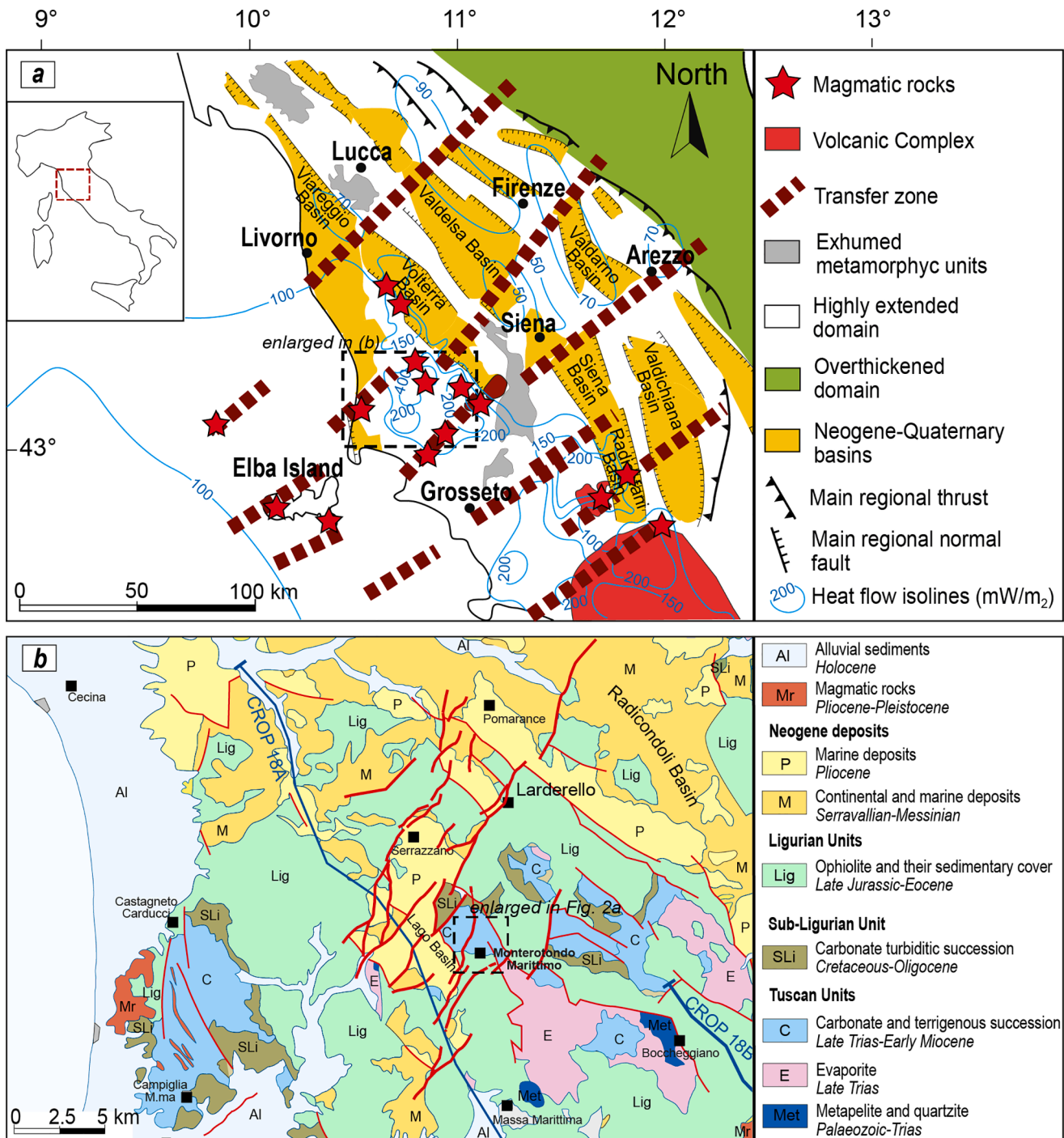
Fig. 1. a) Structural sketch map of the Northern Apennines and Northern Tyrrhenian Sea; b) geological map of the Larderello area (modified after Liotta and Brogi, 2020). The study area is highlighted by the black dashed frame.
