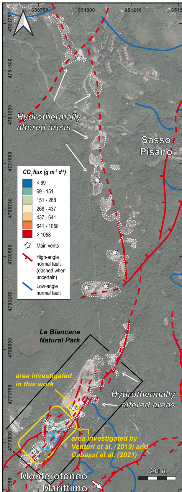
Fig. 3. Hydrothermally altered zones along the Monterotondo Marittimo-Sasso Pisano fault zone. The location of the main faults and hydrothermal vents (after Venturi et al., 2019; Leila et al., 2021; magma database www.magadb.net ) are also reported and the diffuse soil CO 2 measurements by Venturi et al. (2019) and Cabassi et al. (2021) are highlighted.
