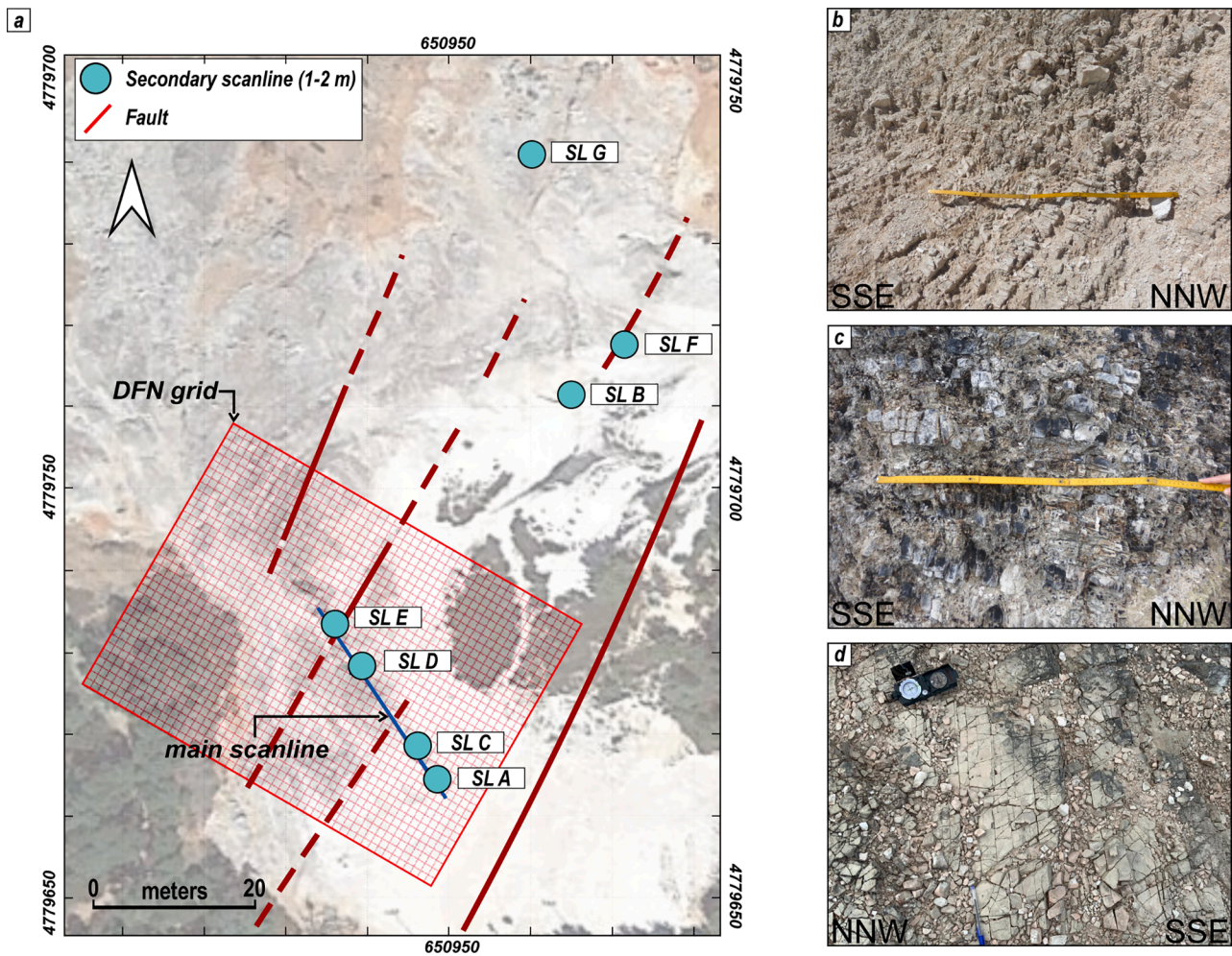
Fig. 5. a) Map showing location of scanlines, DFN grid and the main faults affecting the area. The grid of the DFN model was oriented to follow the main orientation (N30°) of the observed faults. A main scanline (blue line N145° oriented) was performed along the scarp following the better exposure of the fracture and fault networks, as well as the main geothermal manifestations. Secondary scanlines/scan areas (from A to G; turquoise circles) were located along the main scanline (SL A, C, D, E) and the adjacent scarp (SL B and F, N80° oriented). b-c) Examples of fractures measured along scanline A (b), scanline E (c); d) example of fracture setting plain view (SL G), these few spots of pavements (5) were used for performing scan areas.
