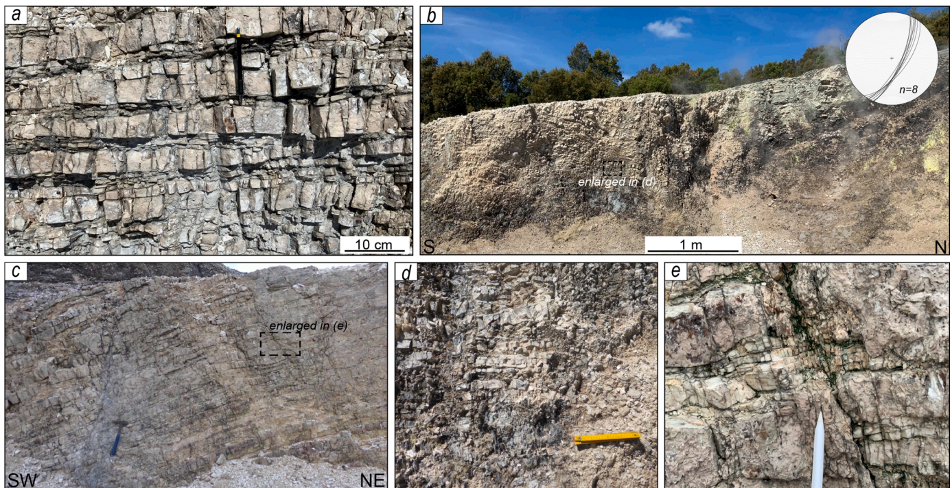
Fig. 8. a) Photograph of the Jurassic siliceous beds (Diaspri Fm) exposed in the study area; b) panoramic view of the main fault zone exposed along the scarp (Fig. 5a); c) panoramic view of a minor fault exposed in the study area; d) detail of the fault zone showing highly fractured and altered (dark zones) Diaspri Fm due to the intense hydrothermal activity occurring along the fault zone; e) detail of the shale and siliceous beds cut by a minor fault.
