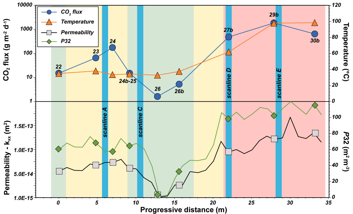
Fig. 14. Soil CO 2 flux, temperature, P32 and permeability measurements carried out along the transect represented in Fig. 12, which runs orthogonally to the MMSF fault zone. The location of the secondary scanlines is also shown in turquoise. Background colors represent the main transport mechanism of CO 2 ; green: diffusive, yellow: mixed diffusive and advective, red: advective.
