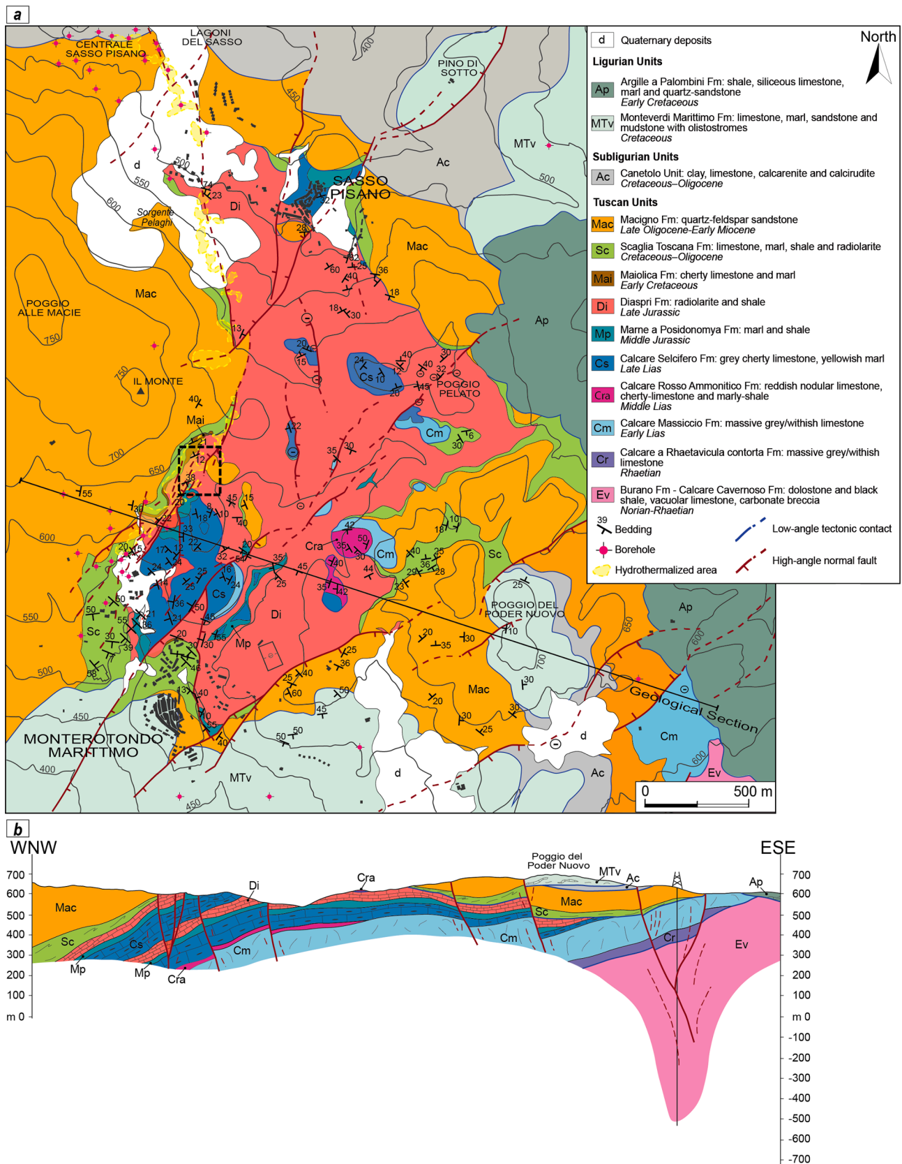
Fig. 2. a) Geological and structural map of the Monterotondo Marittimo-Sasso Pisano (MMSP) area in which the main faults defining the transfer zone and the study area (black dashed frame) are shown; b) geological section across the study area. Its trace is indicated in (a).
