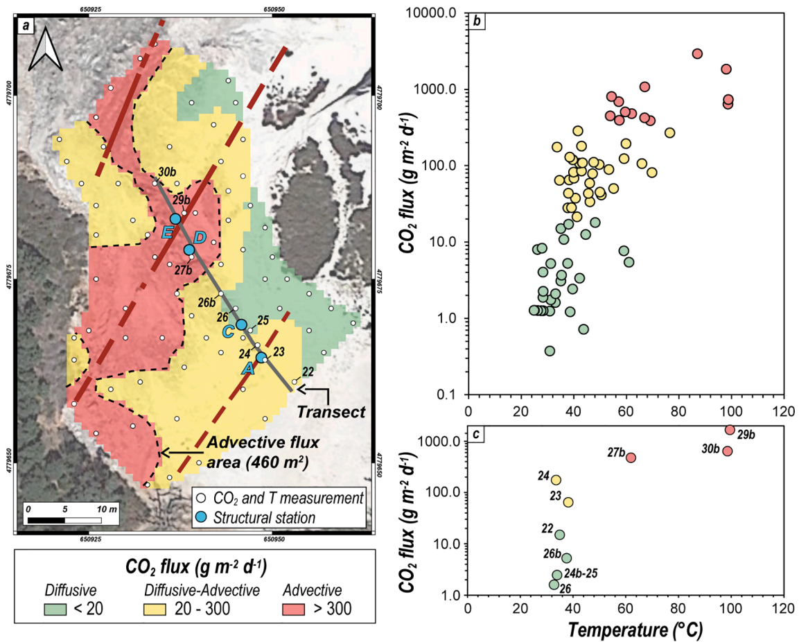
Fig. 12. a) Distribution map of the soil CO 2 flux divided by the inferred transport mechanisms; b) relationship between soil CO 2 and temperature in the study area and c) along the transect in (a). Numbers in (a) and (c) represent the ID of the measurement points reported in the supplementary material.
