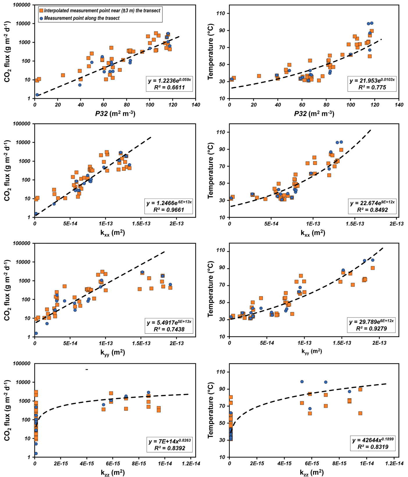
Fig. 13. Correlation among soil CO 2 flux and temperature measurements (blue circles measured, orange squares interpolated) and the DFN modeling outputs (P32, k_{xx} , k_{yy} , k_{zz} ).
