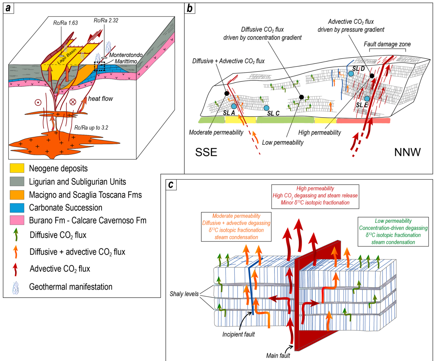
Fig. 15. a) Geological sketch (not to scale) illustrating the tectonic and geothermal context of the Monterotondo-Sasso Pisano area, in the frame of the Lago pull-apart Basin developed within the transfer zone affecting the geothermal area of Larderello; b-c) local (b) and conceptual (c) models of the behavior of the CO 2 and steam emissions and transport mechanism, influenced by the enhanced permeability through the fault zone.
