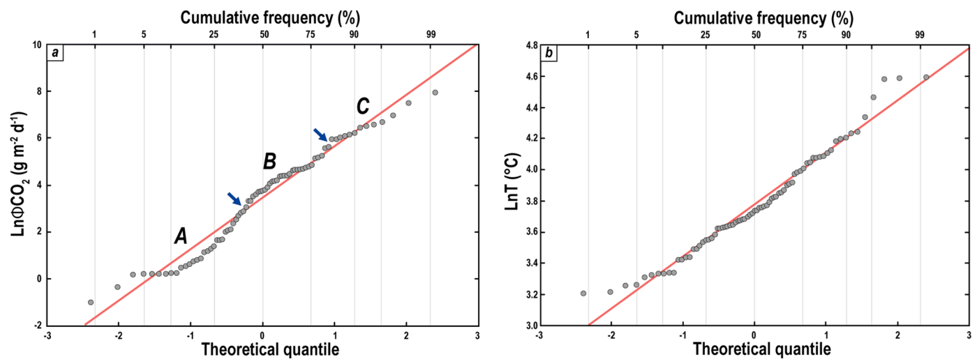
Fig. 6. Cumulative frequency plots of the (a) soil CO 2 and (b) temperature measurements.
