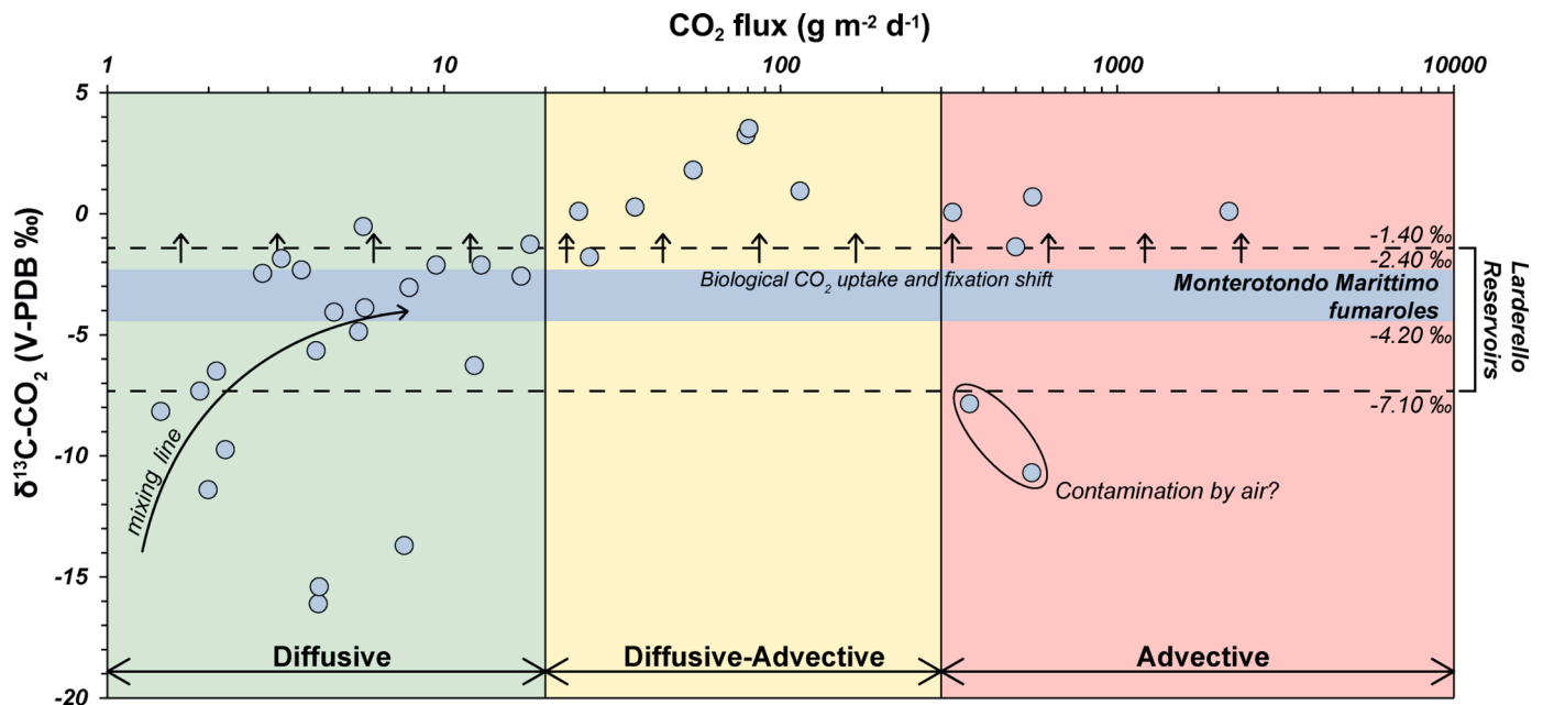
Fig. 10. Soil \text{CO}_2 flux vs. isotopic composition of fluxes from the Monterotondo Marittimo area (data from Venturi et al., 2019). \delta^{13}\text{C}\text{-CO}_2 composition of Monterotondo Marittimo fumaroles (Venturi et al., 2019; Leila et al., 2021) and Larderello reservoirs are also reported (Gherardi et al., 2005).
