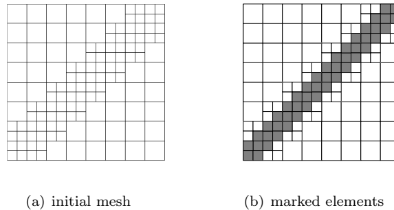
Fig. 4. The admissible meshes in Fig. 1 related to the cases (p_1, p_2) = (i, i) for i = 2, 3, 4 are generated by the call to \mathcal{Q}^* = \text{REFINE}(\mathcal{Q}, \mathcal{M}, 2) to the mesh \mathcal{Q} depicted in (a) with the marked set \mathcal{M} of elements shown in (b).
