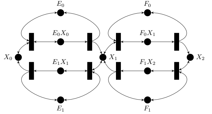
Fig. 3. Double Futile Cycle with distinct enzymes.
