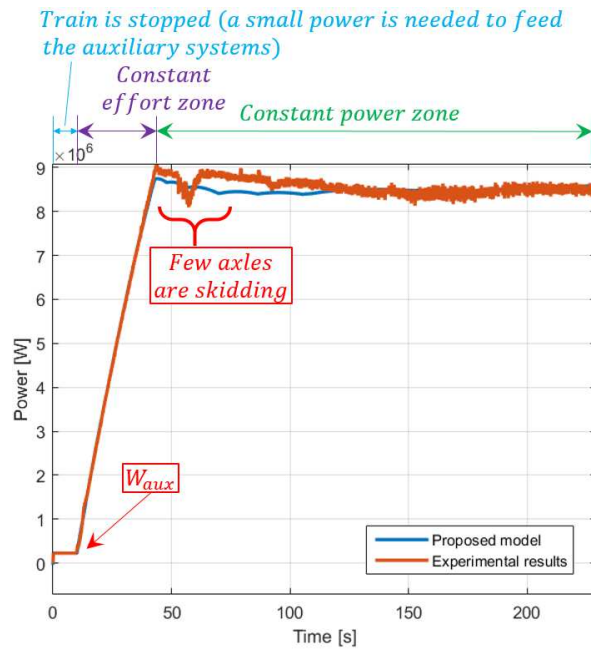
485 Figure 17: Comparison between the experimental power consumption W_e during the traction phase and the corresponding numerical values obtained 486 with the proposed model.
