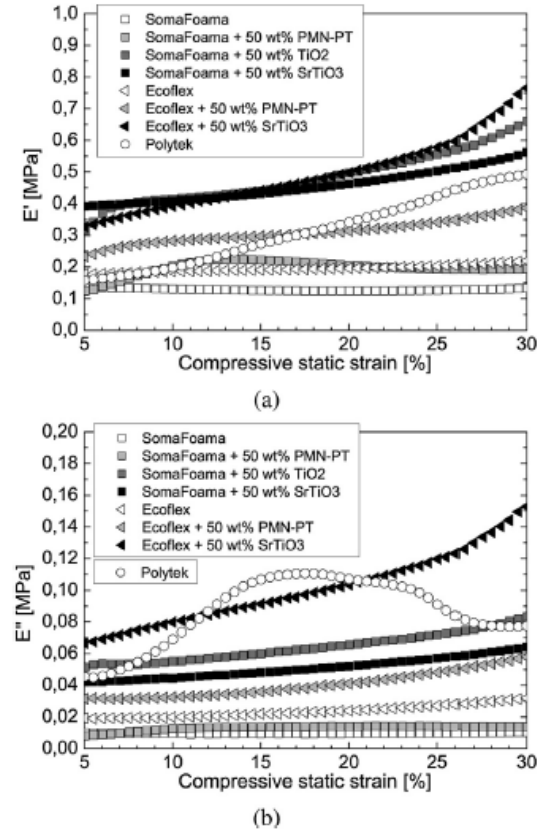
Fig. 4. Storage (a) and loss (b) modulus as a function of the applied compressive strain.
