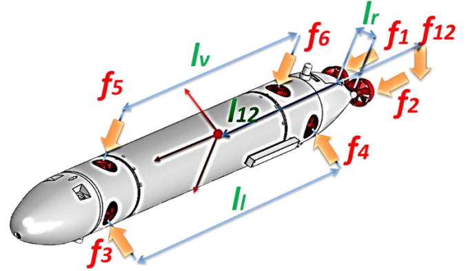
Figure 24: forces exerted by the rear propellers and the thrusters
