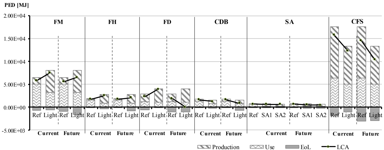
Figure 17 Results of PED [MJ] impact assessment
