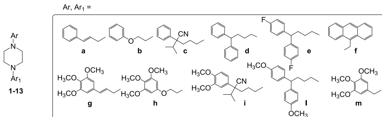
Chart 3. General structure of the newly synthesized piperazine derivatives
