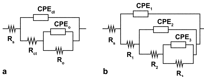
Fig. 10. Electrical equivalent circuits used for quantitative evaluation of EIS spectra. (a): for untreated and 360-°C nitrated samples, and for 380-°C nitrated AISI 316L and AISI 202 samples; (b): for 380-°C nitrated P558 samples.
