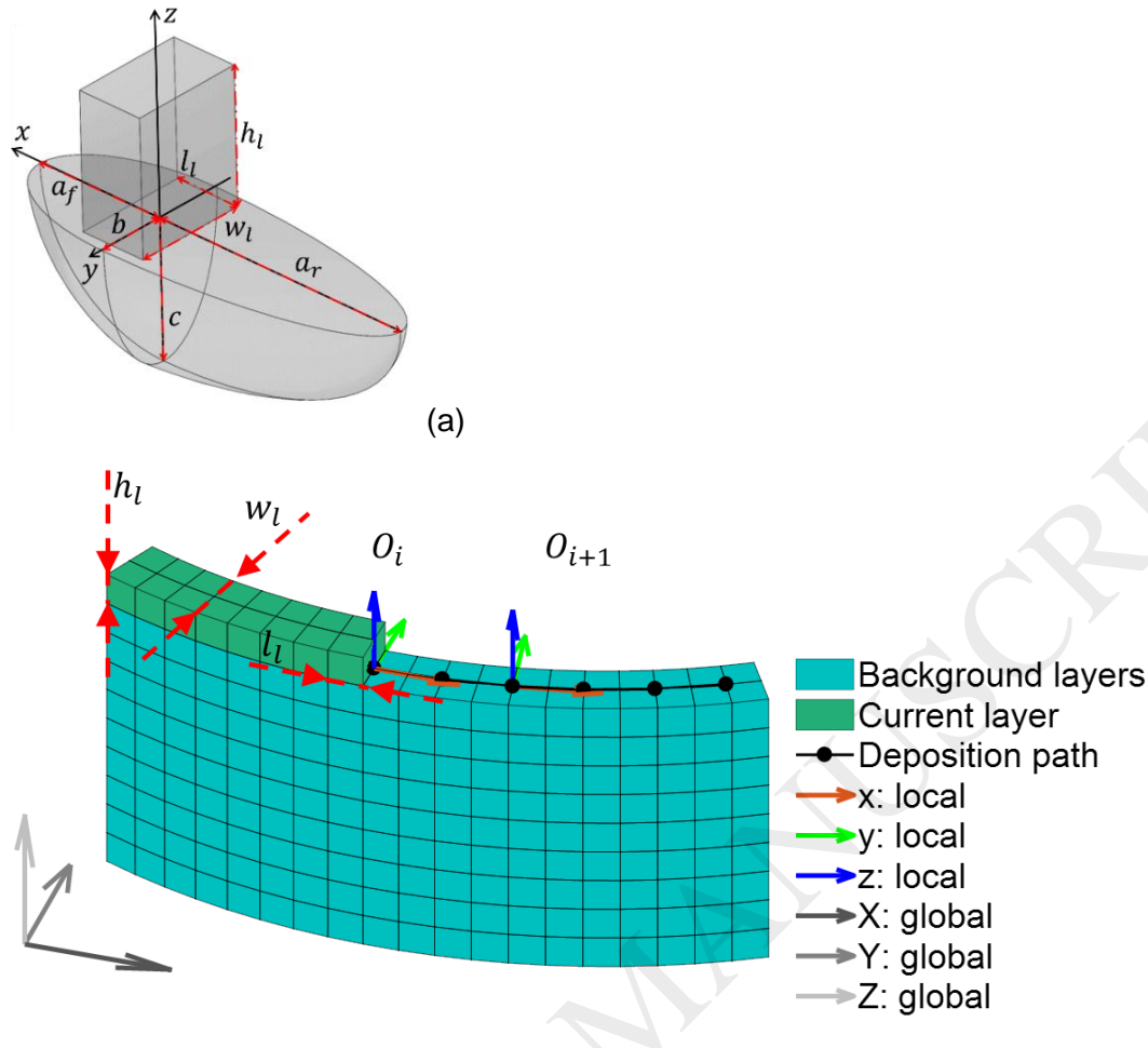
Figure 1: Heat source model used for WAAM simulation (a); Moving coordinate system used in the heat source definition (b).
