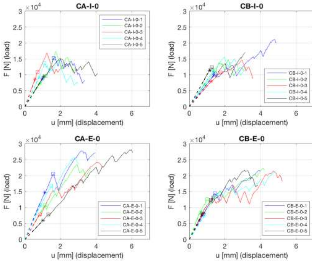
Figure 11: Experimental load-displacement diagrams; * and □ correspond respectively to first cracks ( P_f ) and first peak ( P_1 ) points.
