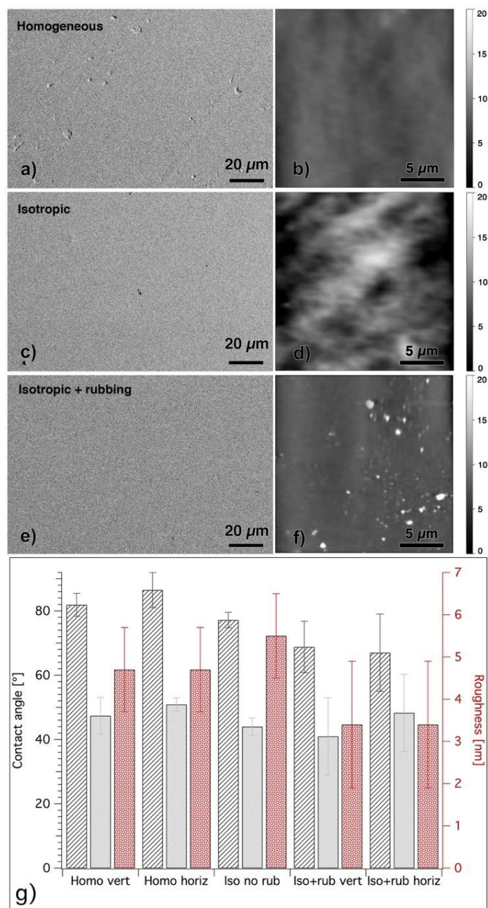
Figure 3. Material surface characterization. SEM (left, a, c, e) and AFM (right, b, d, f) micrographs of homogeneous, isotropic and isotropic (made in the rubbed cell) samples. g) Advancing and receding contact angle (grey bars) and roughness value (red bars, right y-axis) of the analyzed samples: the rubbed samples were investigated in vertical and horizontal directions
