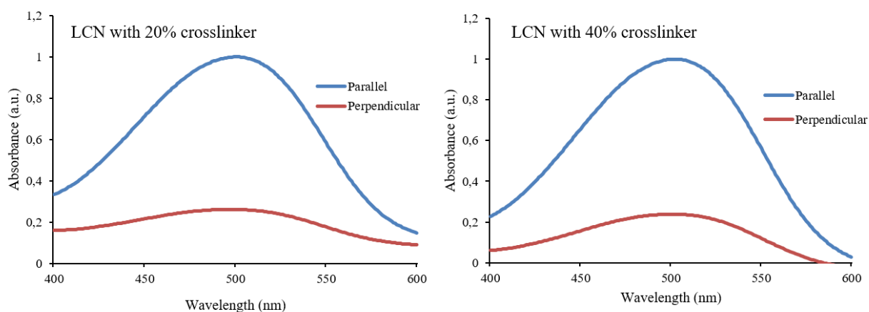
Figure S4. Polarized absorption spectra of LCNs with planar homogeneous alignment recorded respectively in parallel and perpendicular directions with respect to the nematic director.
