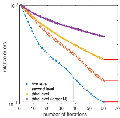
Fig. 13: The residuals of the misfit at different levels. The residuals drop to 10%, 17%, 30% of the starting value at the first, second and third levels, respectively. The purple line shows the residual decay with a much larger N = 61448 at the third level. Y-axis is on the log scale. The red lines show that the residuals reach the stopping criteria.
