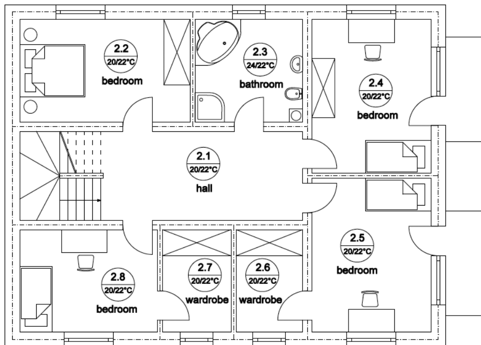
Fig. 2. First floor
