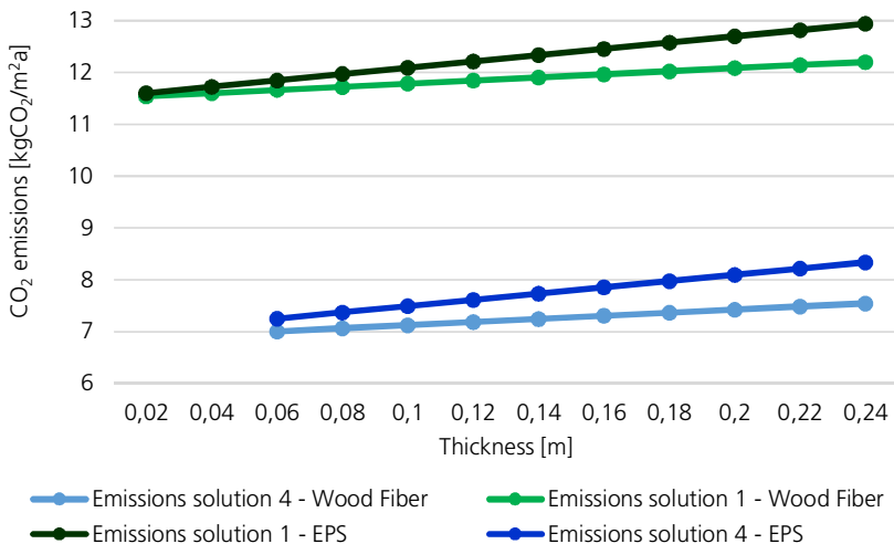
Fig. 6. CO 2 emissions of technological solutions 1 and 4.
