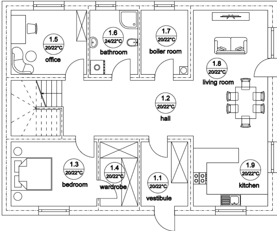
Fig. 1. Ground floor
