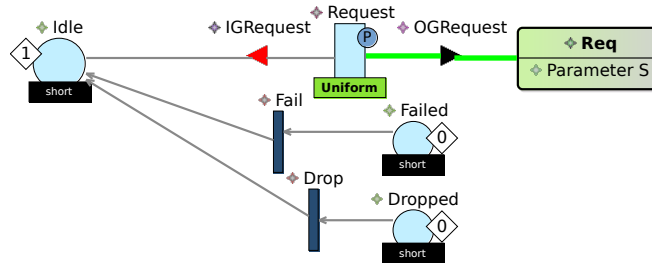
Fig. 6. Example of a SAN-T model, specified with our editor. Request , OGRRequest , and Req are template-level entities, and thus highlighted in green.
