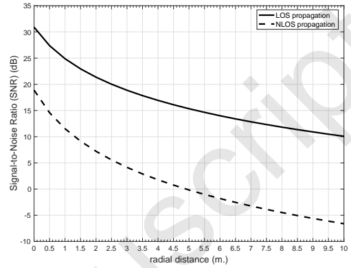
Figure 7. Measured SNR vs. radial distance for the SIW antenna array
