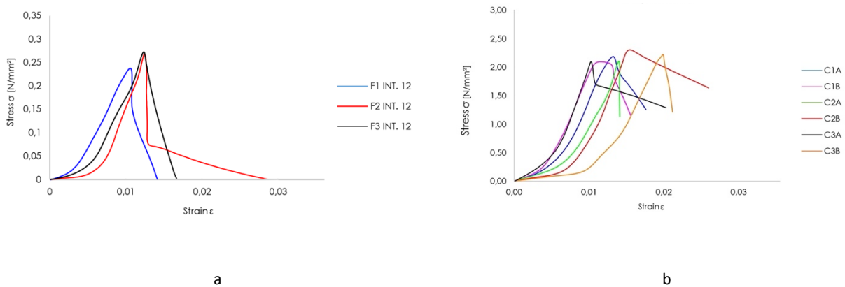
Figure 3. Results obtained on the I2 thermal mortar in relation to: a) flexural tests; b) uniaxial compression tests
