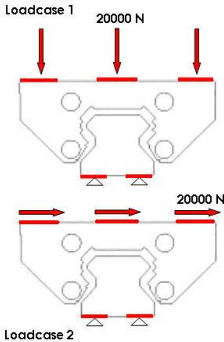
Figure 11: Exemplary cross-section of the linear guidance and typical applied loads [22].
