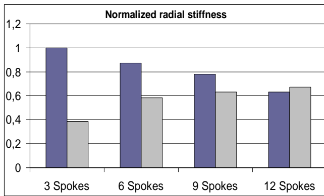
Figure 7: Normalized radial stiffness distribution evaluated on the wheel rim for different topologies: radial force applied on the spokes (dark) and in the middle between two adjacent spokes (light)
