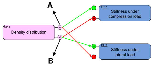
Figure 13: Geometrical contradiction: “A” is topology coming from optimization under load case 1, “B” is topology resulting from optimization under load case 2.
