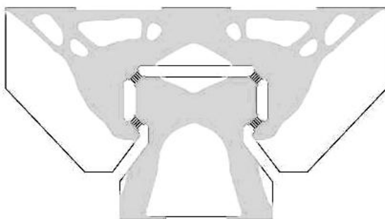
Figure 15: Topology resulting from multi-objective design optimization according to the objective function (3) under a mass constraint equal to the hybrid topology (figure 12-B).
