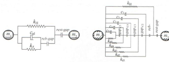
Figure 6: Finite element schematization of Herzdamp model (left), and multi-damper model elaborated in this study for the analysis of pounding impact.
