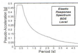
Figure 8: BDE-scaled pseudo-acceleration elastic response spectrum.
