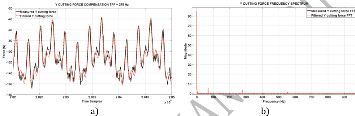
Fig. 11. Cutting test 2, Y direction measured and compensated forces: time domain (a) and frequency domain (b) comparison.
